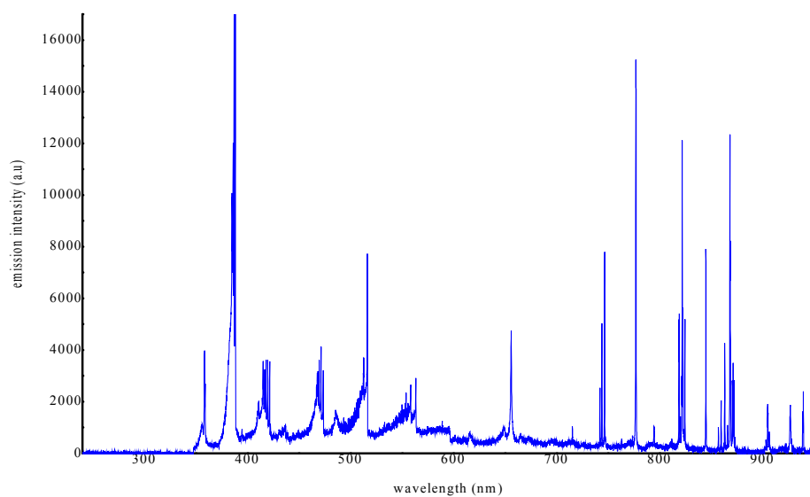
Fig. 3. Typical LIBS emission spectrum of the crude oil (Adaril B) sample
