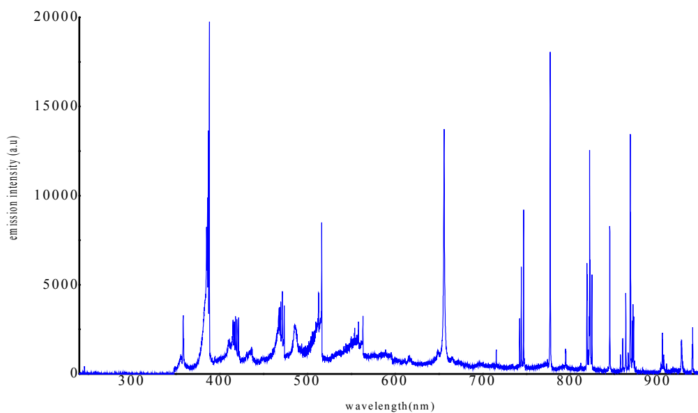
Fig. 4. Typical LIBS emission spectrum of the crude oil (Adaril C)
